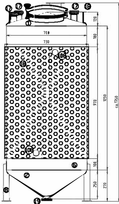
Detail Pos.8
